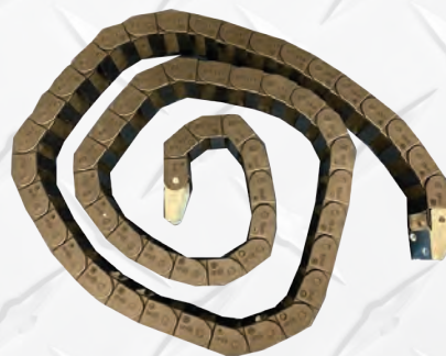
Hose Track Series 10/12 Chevron car carrier, Autogrip.
